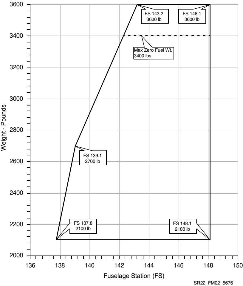
Figure 2-1: Center of Gravity Envelope
