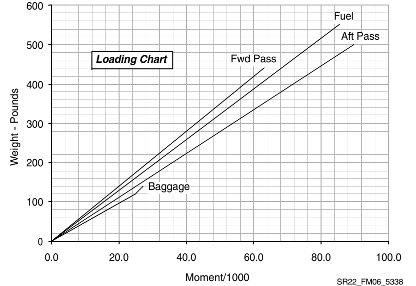
Figure 6-3: Loading Chart
